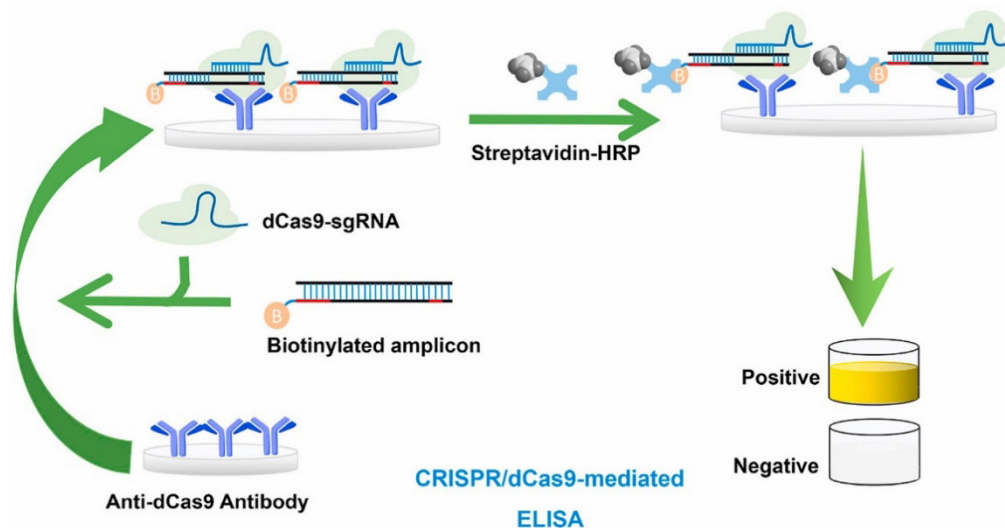
Figure 4) A diagram of the mechanism of action of CAs that perform recognition based on target binding (cas9 and dcas9) [19]
