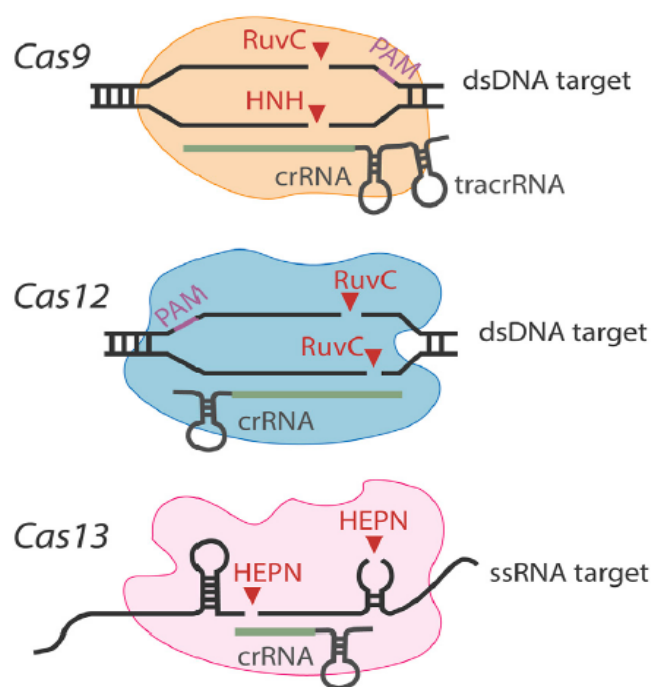
Figure 5) Illustration of the three Cas proteins and their structural regions active in nucleic acid cleavage [24]. Cas9 is structurally composed of two lobes: the nuclease lobe (NUC) and the recognition lobe (REC). The NUC lobe contains two endonuclease domains, HNH and RuvC, along with a PAM-interacting domain. Cas12 contains only a RuvC-like domain, and Cas13 contains two higher eukaryotic and prokaryotic nucleotide-binding domains (HEPN) for nucleic acid cleavage
