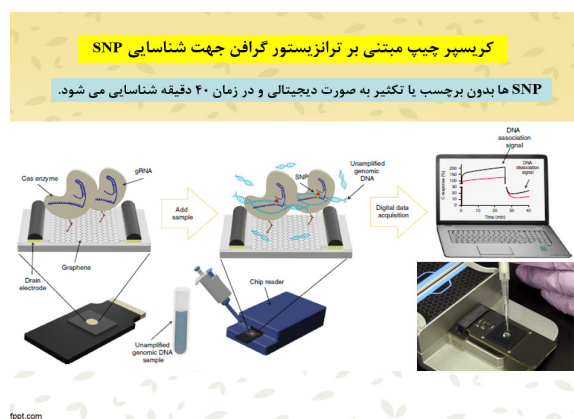
Figure 8) Image of using CRISPR chip to detect SNPs that can be used for identification and criminology [27]
